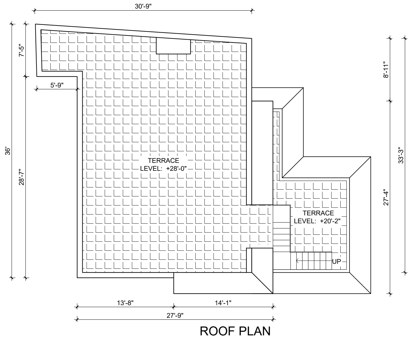
ROOF PLAN
