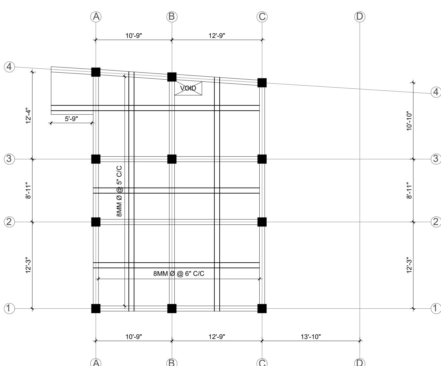
SLAB BOTTOM REINFORCEMENT LAYOUT PLAN (TOP FLOOR)
