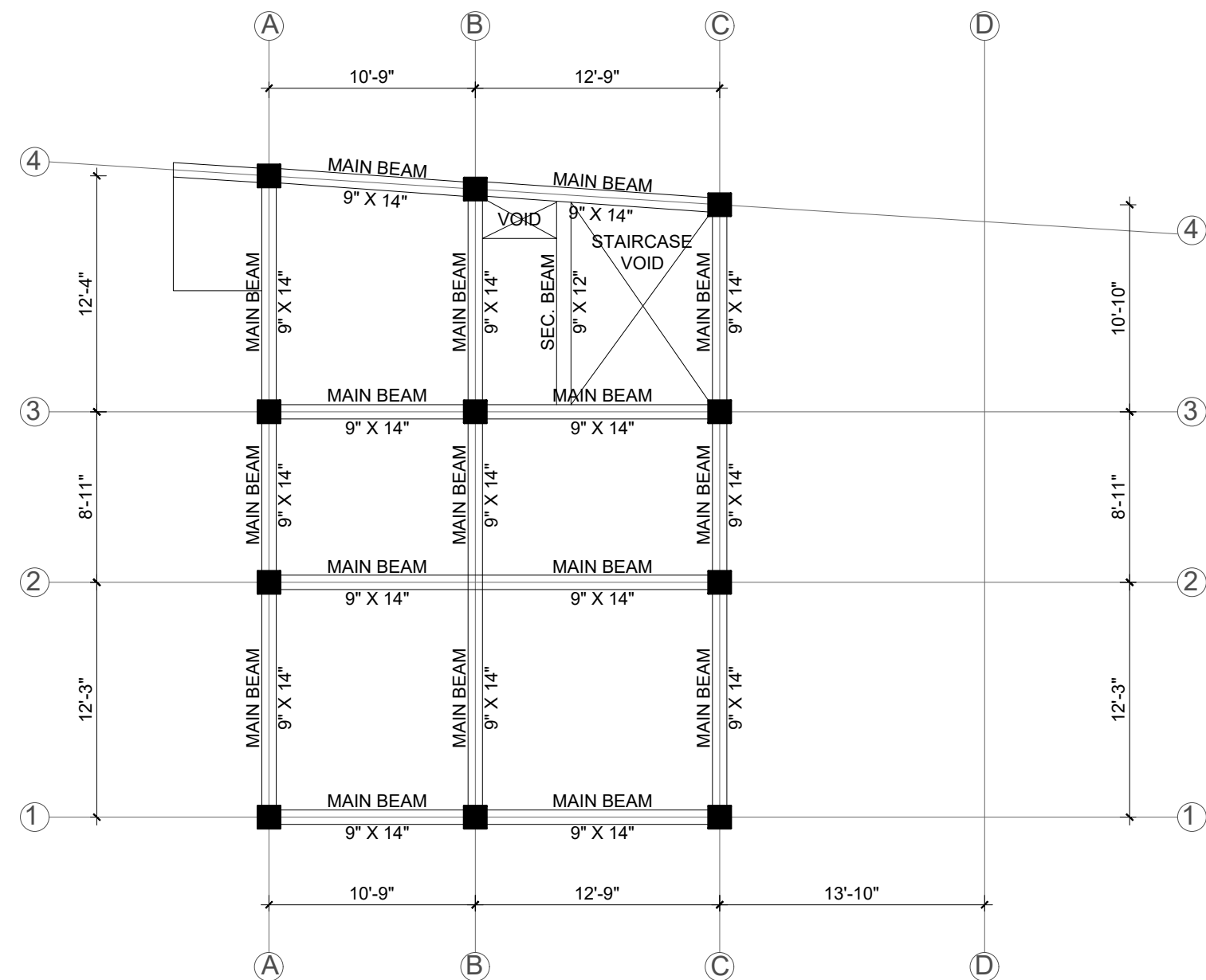
BEAM LAYOUT PLAN (TOP FLOOR)
