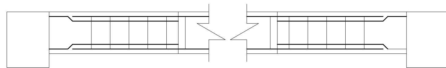
BEAM LAPPING DETAILS
