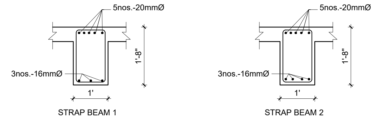
S. No. GRID Footing Size Strap Beam Width Strap Beam Depth Rebar Detail Length L1 Breadth(m) B1 Length(m) L2 Breadth(m) B2 1. GRID A (4-3) 5'-0" 5'-6" 6'-6" 5'-6" 12" 20" 5-20mm reinforcement@top and 3-16mm reinforcement@bottom 2. GRID B (4-3) 5'-0" 6'-8" 7'-8" 6'-8" 12" 22" 5-20mm reinforcement@top and 4-16mm reinforcement@bottom 3. GRID C (4-3) 5'-0" 6'-8" 7'-8" 6'-8" 12" 22" 5-20mm reinforcement@top and 4-16mm reinforcement@bottom
