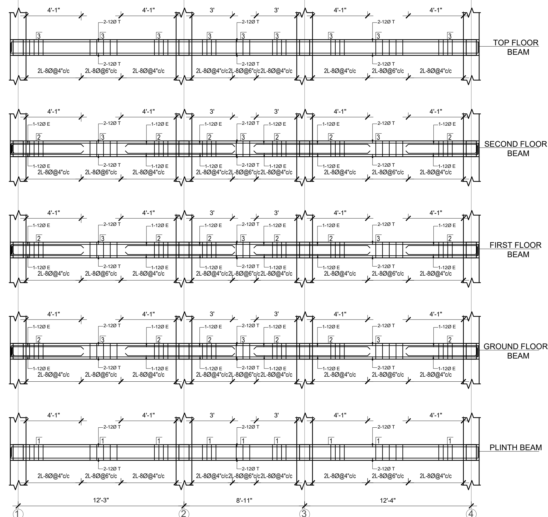
BEAM ELEVATION THROUGH A-A
