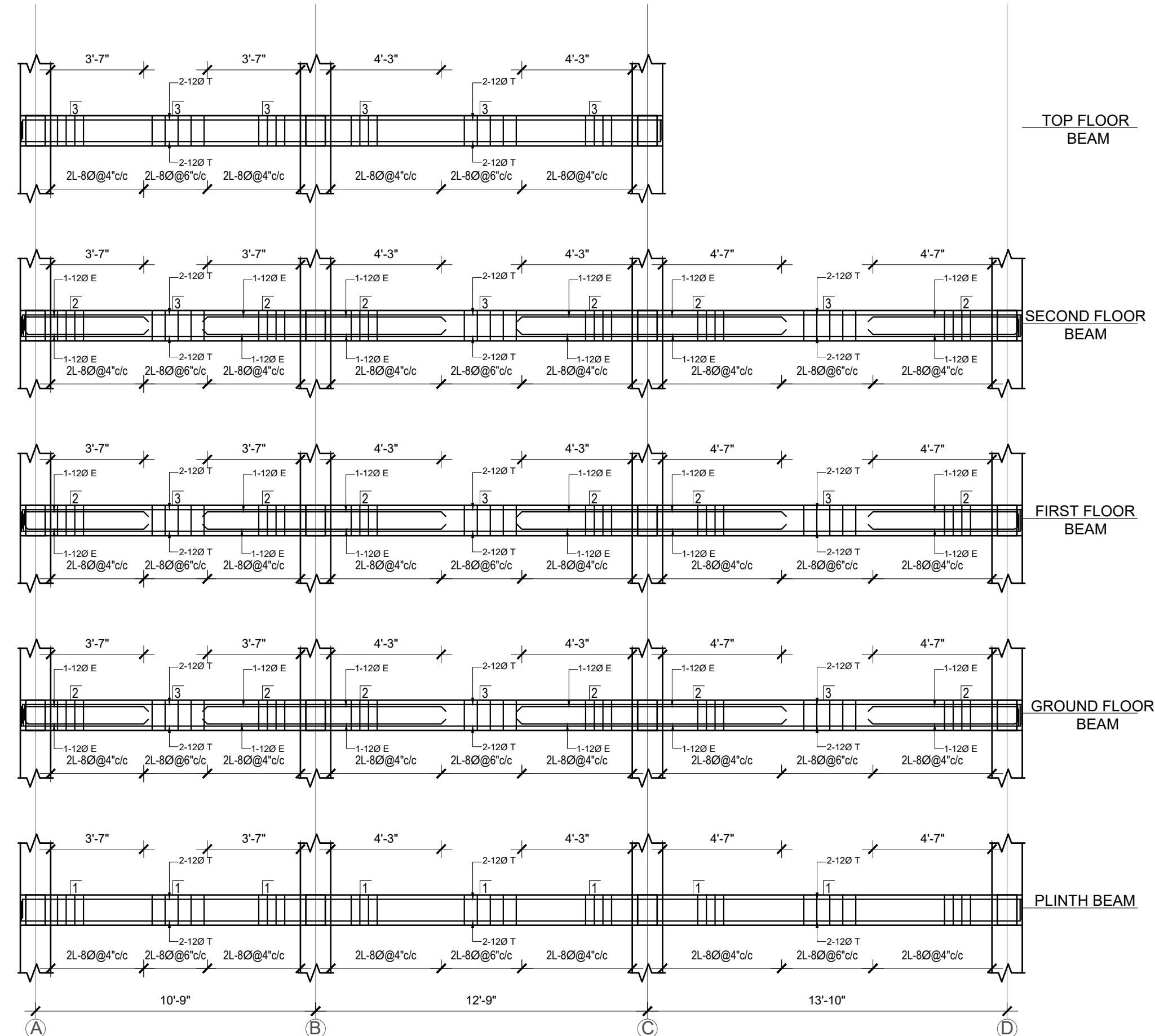
BEAM ELEVATION THROUGH I-1
