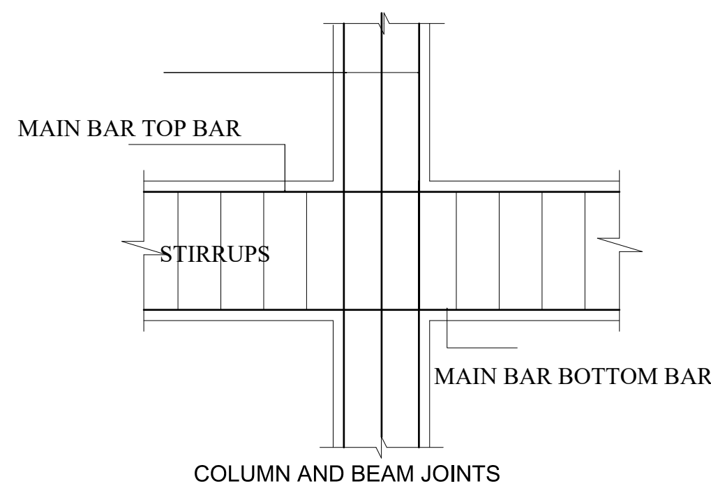
COLUMN AND BEAM JOINTS
