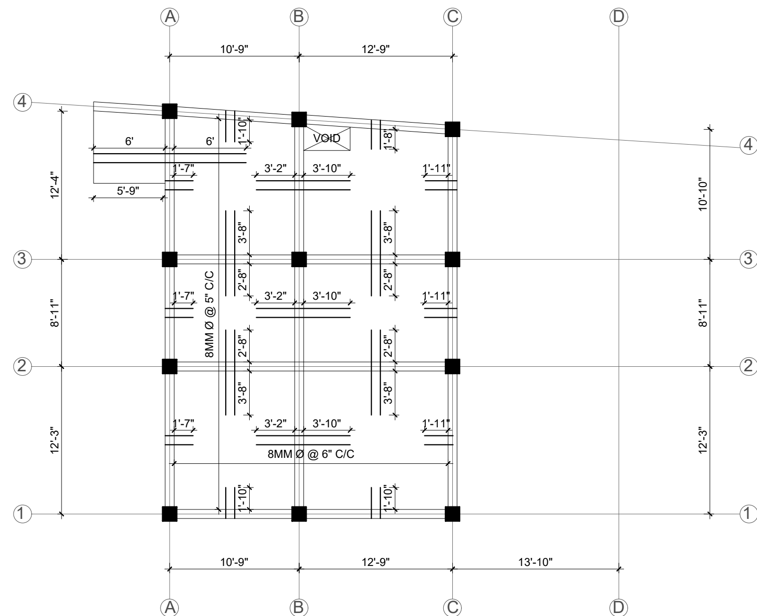
SLAB TOP REINFORCEMENT LAYOUT PLAN (TOP FLOOR)
