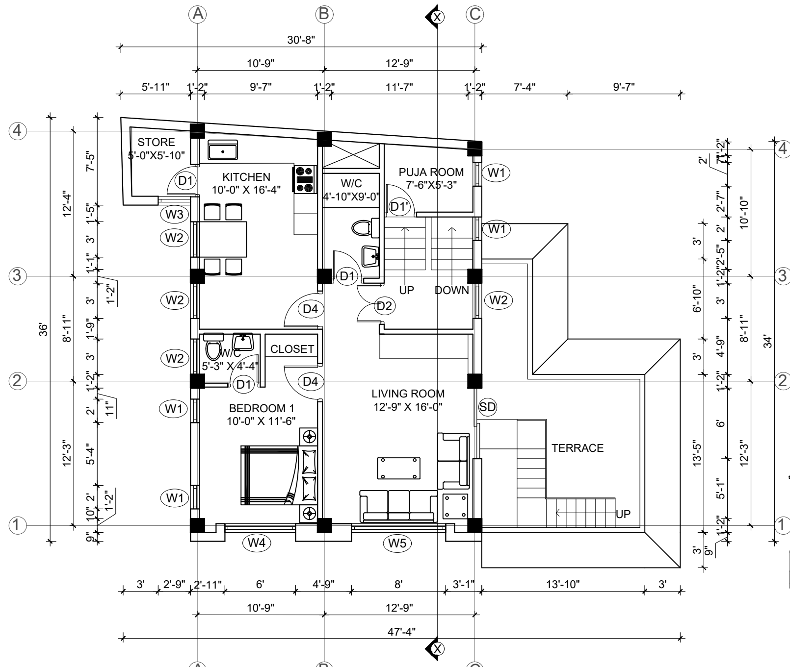
TOP FLOOR PLAN FLOOR AREA: 884.14 SQ.FT
