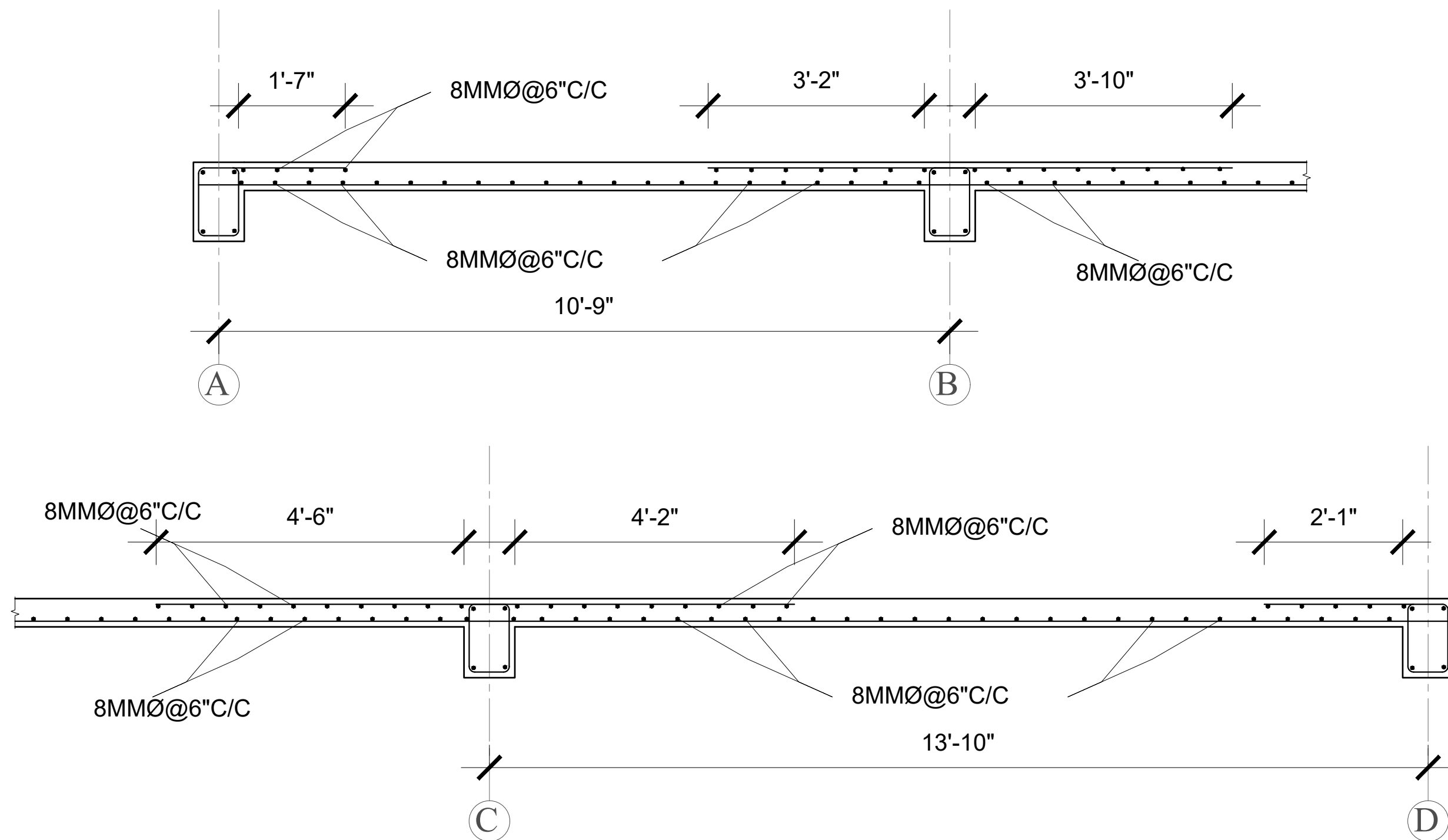
TYPICAL SLAB SECTION AT 1-1
