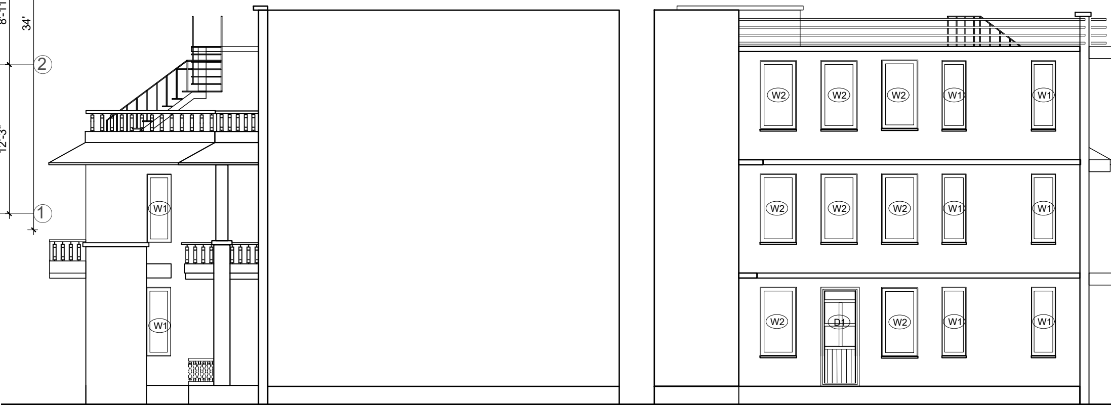
NORTH ELEVATION
