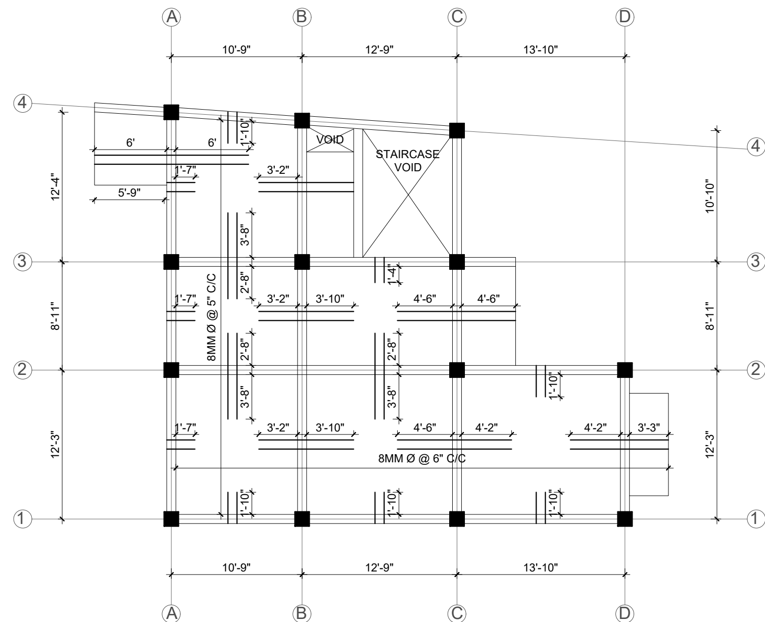
SLAB TOP REINFORCEMENT LAYOUT PLAN (GROUND AND FIRST FLOOR)
