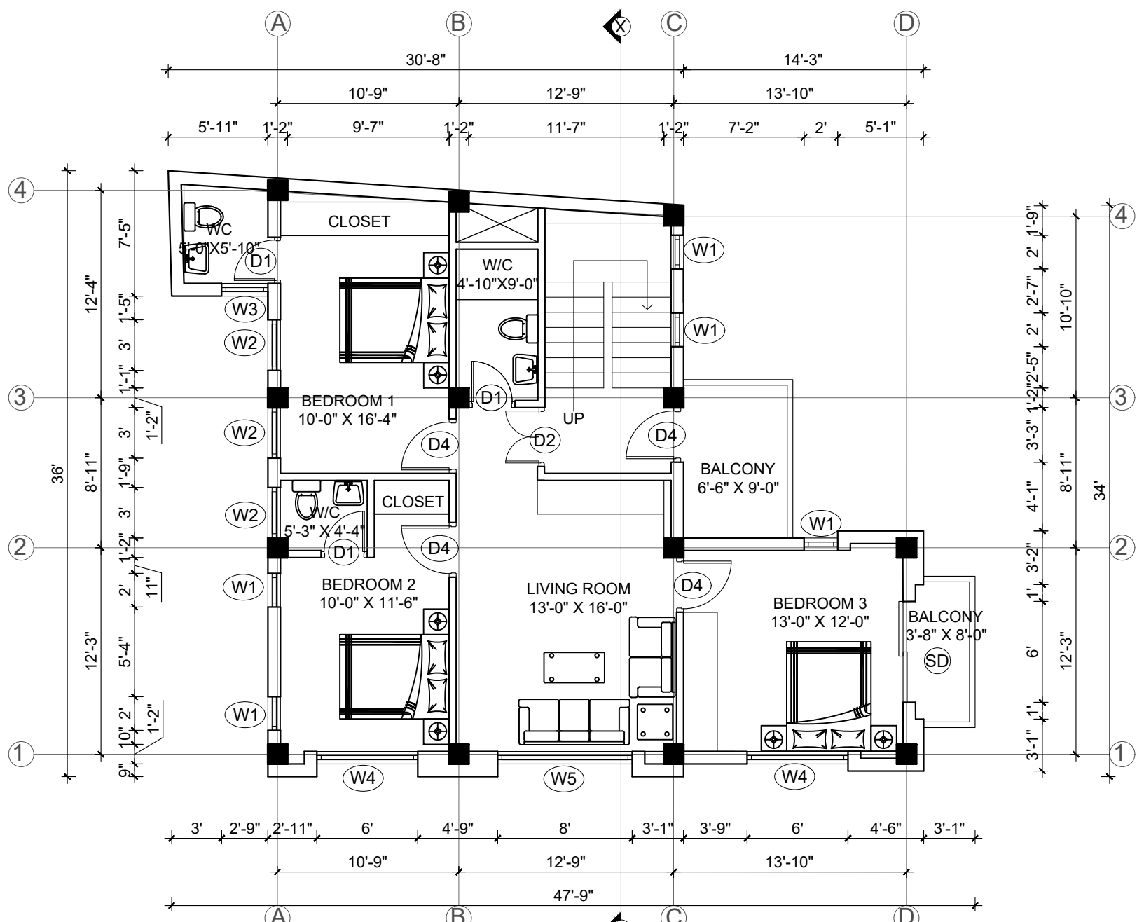
FIRST FLOOR PLAN FLOOR AREA: 1085.42 SQ.FT
