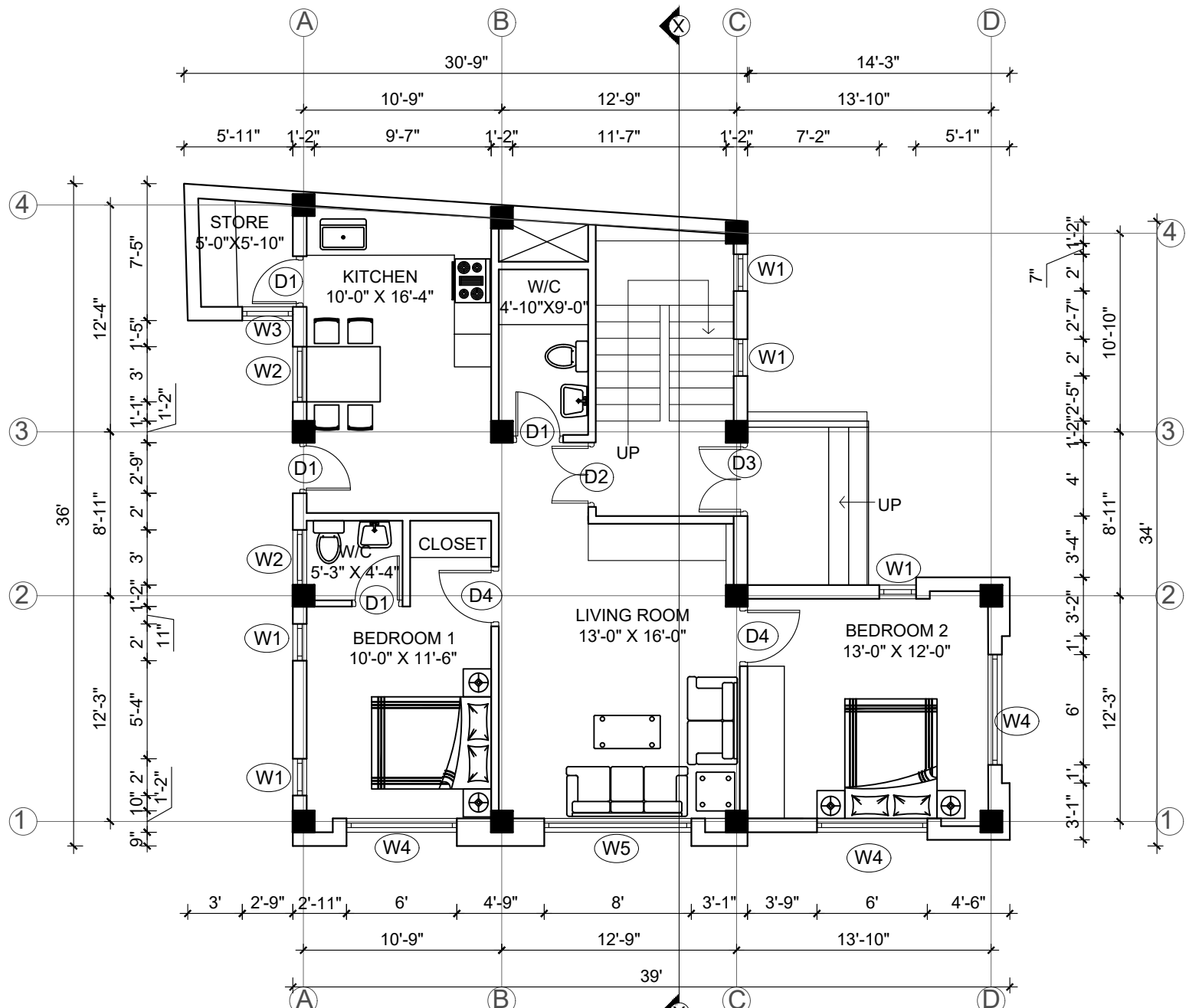
GROUND FLOOR PLAN FLOOR AREA: 1085.42 SQ.FT
