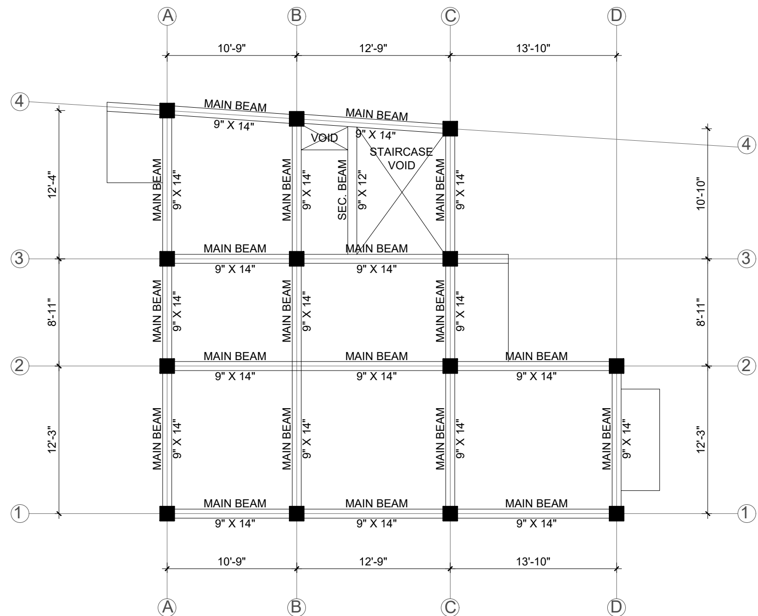
BEAM LAYOUT PLAN (GROUND, FIRST AND SECOND FLOOR)
