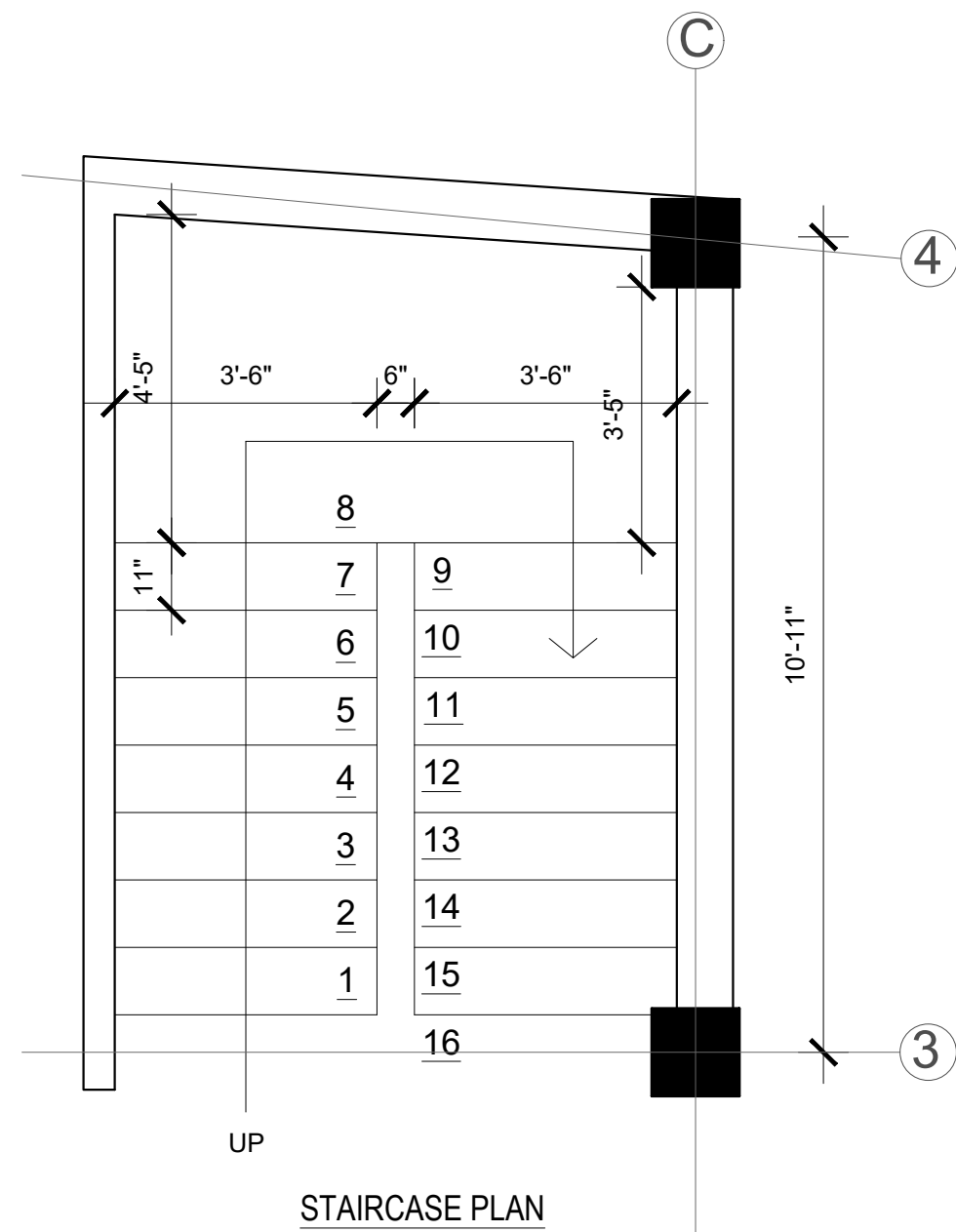
STAIRCASE PLAN
