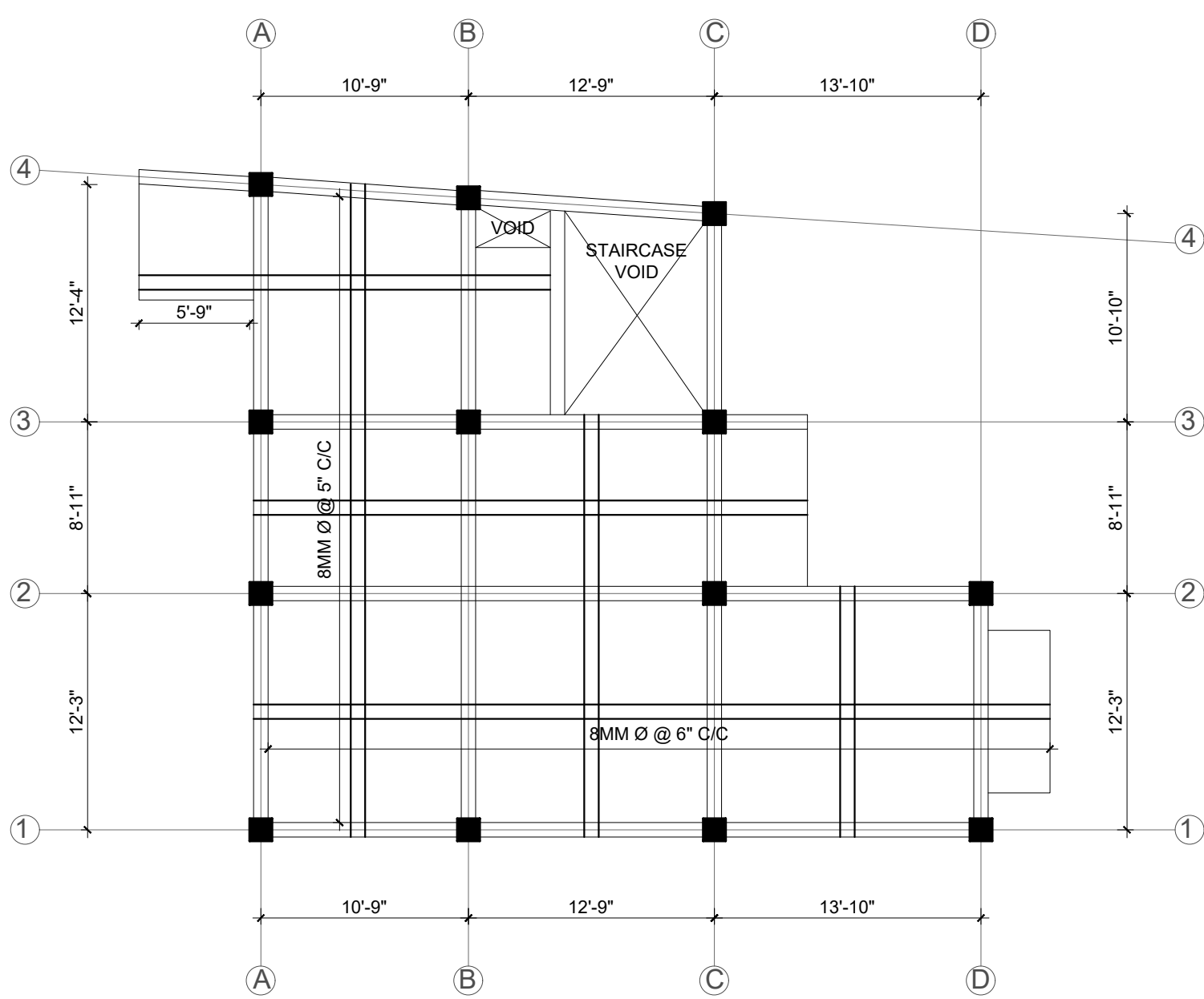
SLAB BOTTOM REINFORCEMENT LAYOUT PLAN (GROUND AND FIRST FLOOR)
